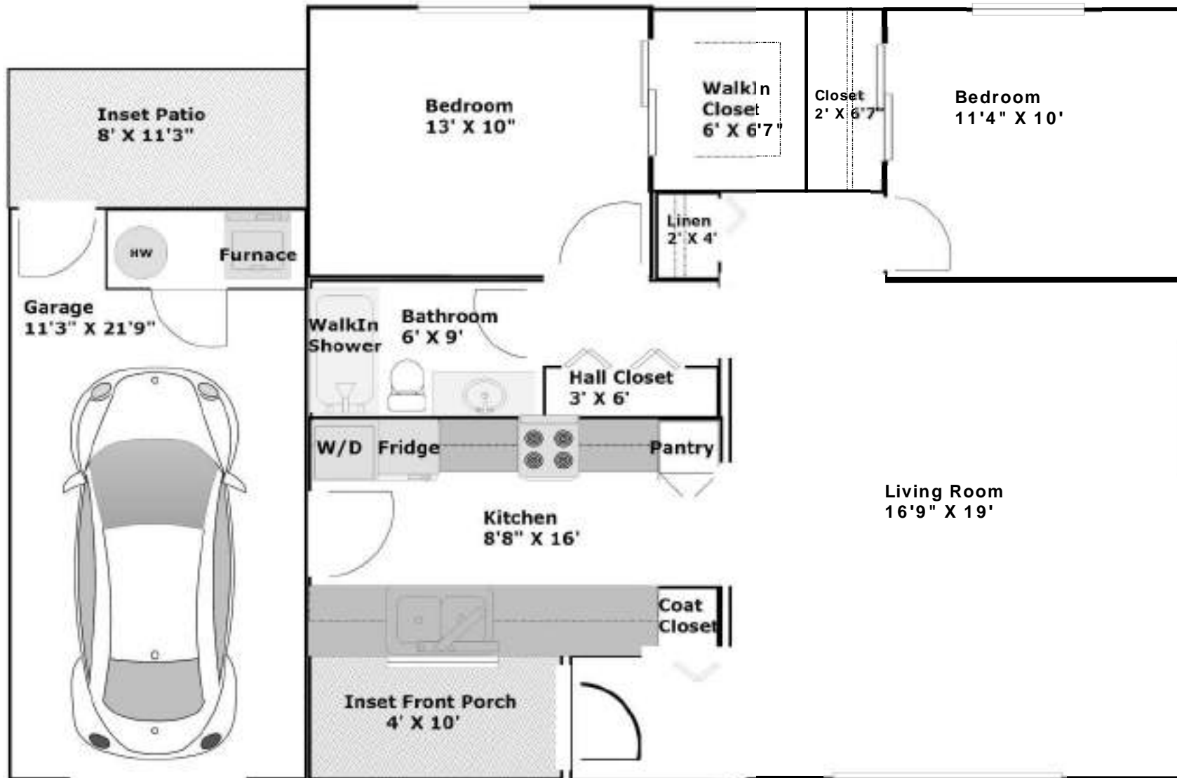
LINCOLN FLOOR PLAN, 2 BED, 1 BATH, 930 sq ft
